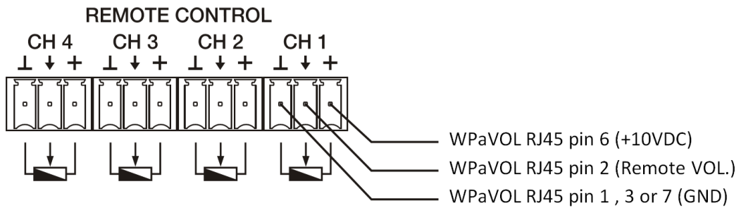
Connection of WPaVOL-SR to remote-control ports
